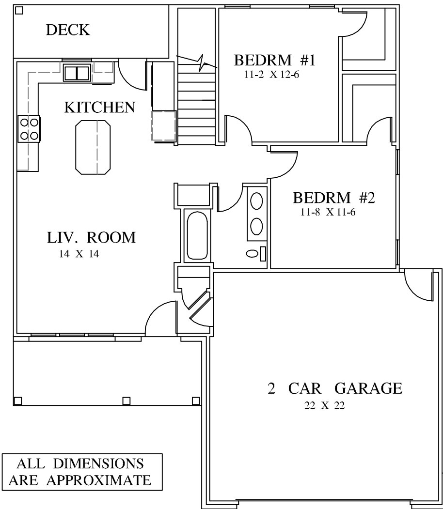
MAIN LEVEL FLR. PLAN 40 X 47
