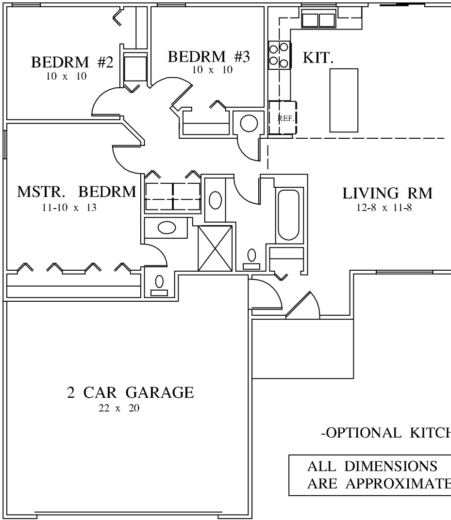
MAIN LEVEL FLR. PLAN 40 x 45-8
