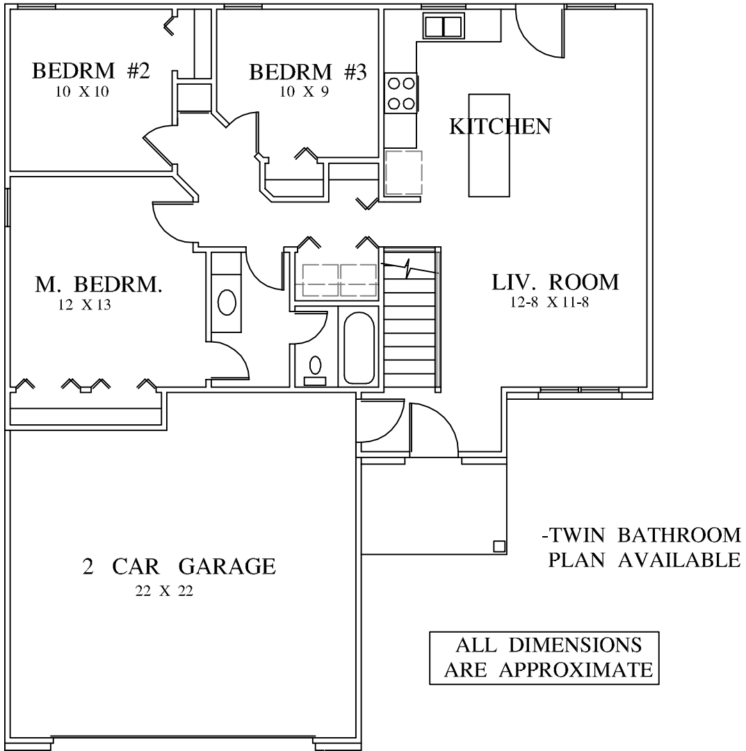
MAIN LEVEL FLR. PLAN 40 X 46
